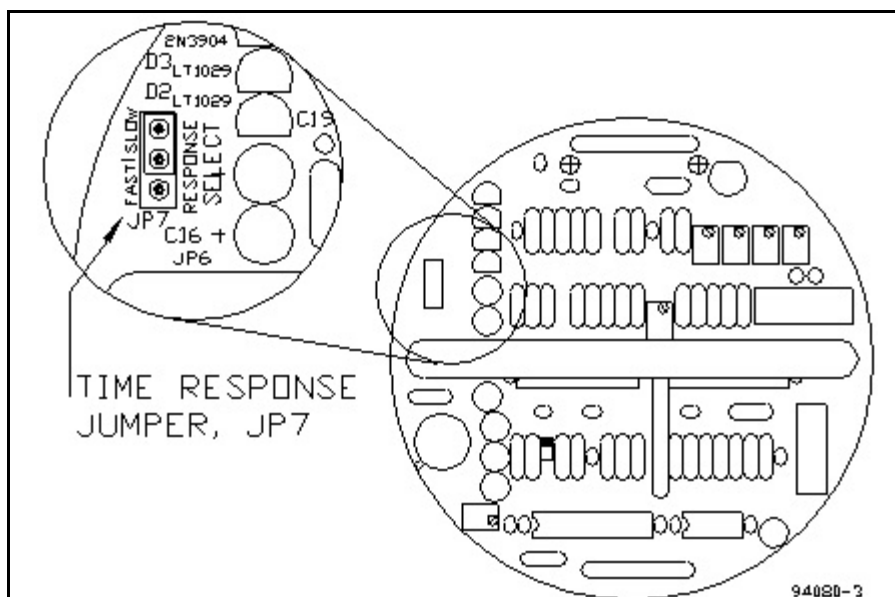
Figure 4. Time Response Selection Jumper Location
