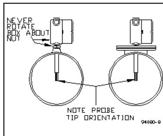
Figure 1. Intrusive Probe Installation.
